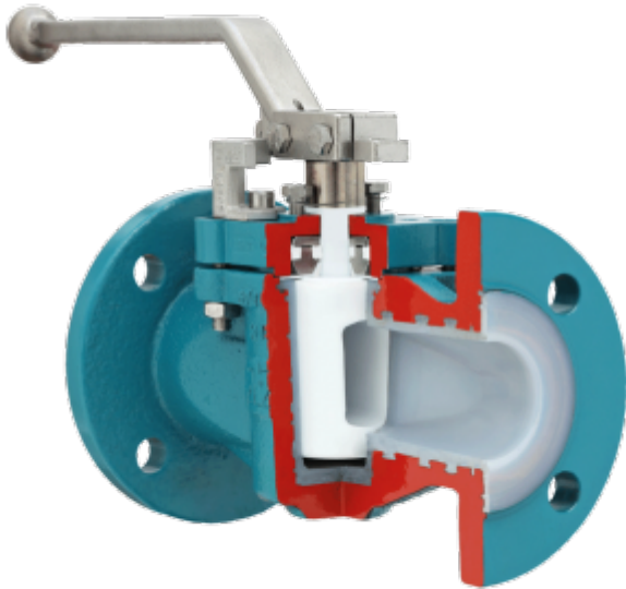
lined plug valve with chemical seal TYPE ISO-STD-A-CA
