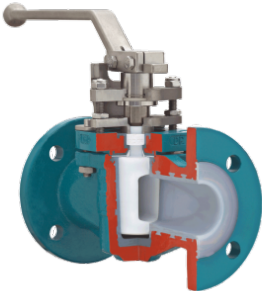
lined plug valve fluctuation temperatures chemical safety seal TYPE SAFE-LINED
