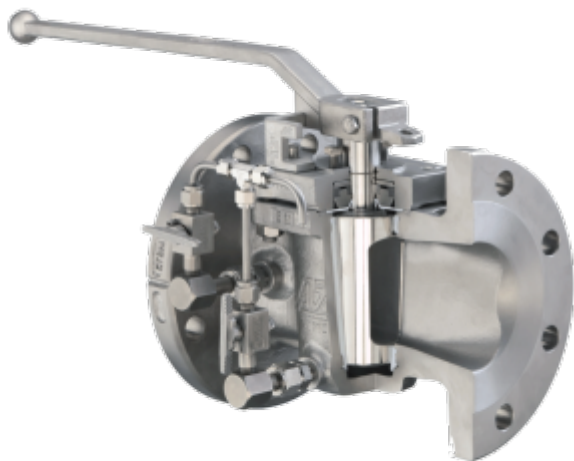
Double Block & Bleed Inspection TYPE DBI
