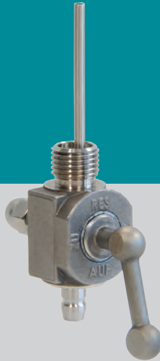
Type VINTAGE fuel valve with reserve option
